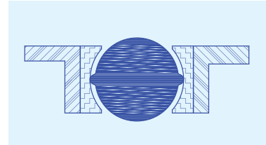
Lionsele® SP Piston seal
